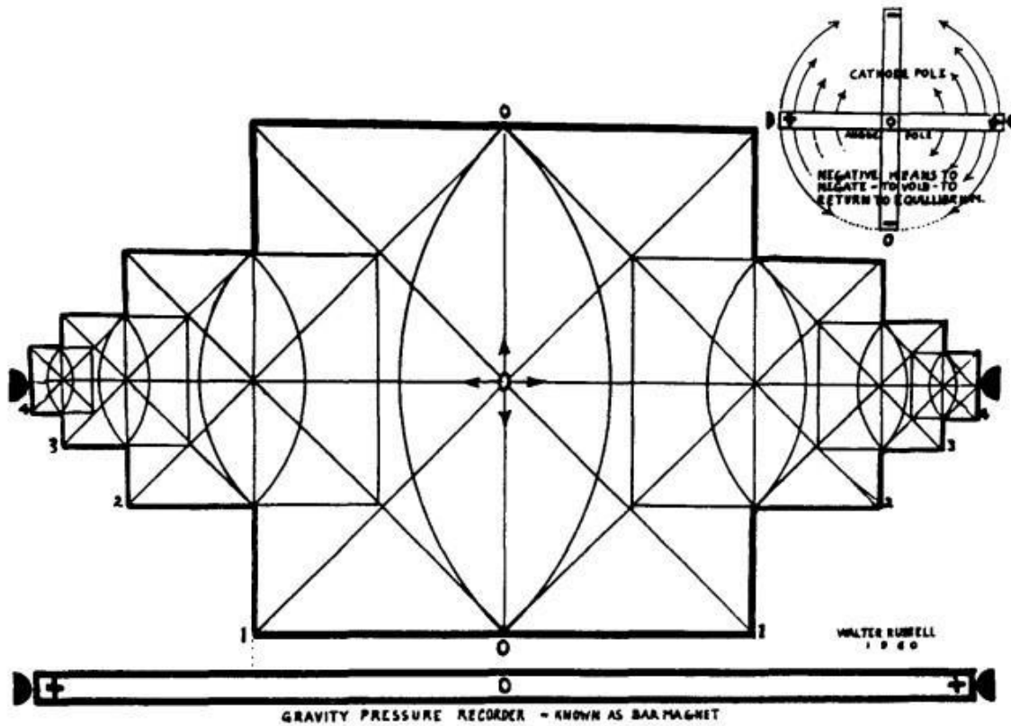
FIG. 58 This diagram represents the compression principle which is created by a series of biconvex lenses which are located on the wave axis at distances apart in inverse of the cube in volume and the square of the distance in length. Always visualize this compression principle when you think of the wave.
